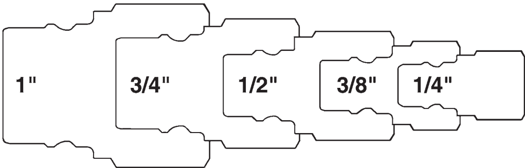
Plug Profiles
