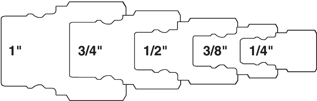
Plug Profiles
