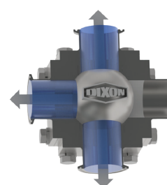
4-way 'T'-port position D
