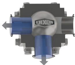
3-way 'L'-port position A
