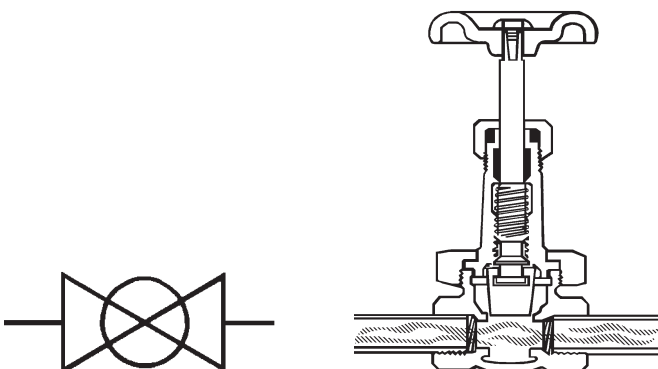
Gate Valve
