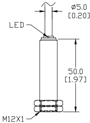
Figure 3 - DW-AS-501-M12
