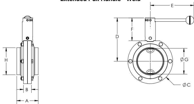
Extended Pull Handle - Weld
