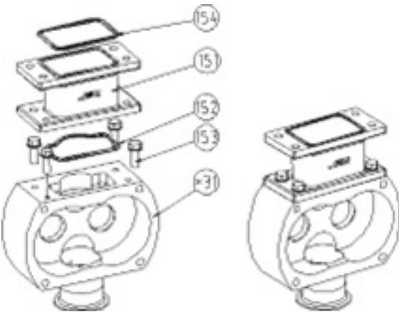
Rectangular Inlet
